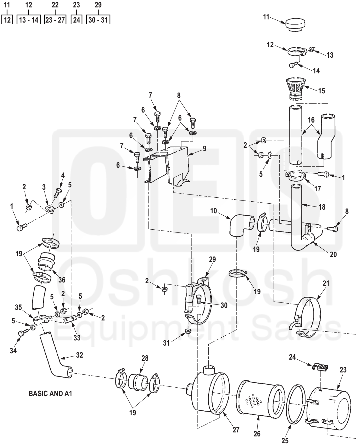
Figure 62. Air Intake System.
